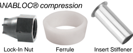
Lock-In Nut
